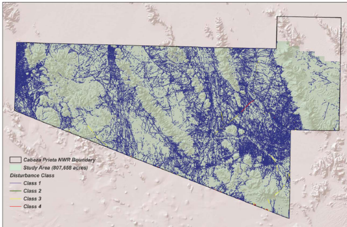
Figure 5. Unauthorized vehicle routes documented within the CPNWR as of November 2008
