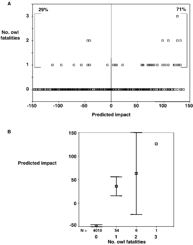
Figure 9. Using our empirical model, we predicted 71% of the wind turbines known to have killed burrowing owls were more likely to kill owls, that is, (A) predicted impact >0 , and (B) our predicted impacts ( \bar{x} and 95% CI) increased with the actual number of owls killed by the wind turbine in the Altamont Pass Wind Resource Area, California, USA, 1998–2003.
